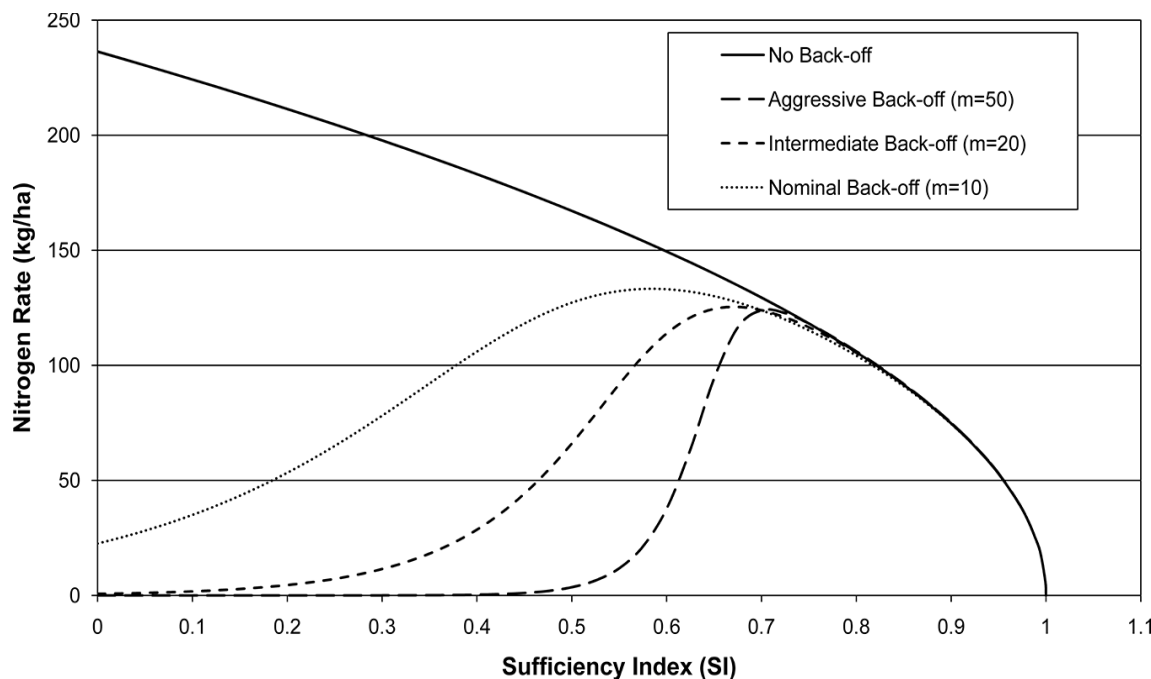
Fig. 7. Comparison of simulated N application using the proposed algorithm incorporating a sigmoidal back-off function. The simulation used an N_{OPT} value of 130 kg N ha -1 . Back-off function was implemented to limit N application for SI values < 1 - \Delta SI. Note, parameters in Eq. [16] are set as follows: MZ_i = 1.0 , N_{PreFert} = N_{CRD} = 0 , NUE = 0.5 , N_{OPT} \approx 0.45 , SI_{Threshold} = 0.7 .
